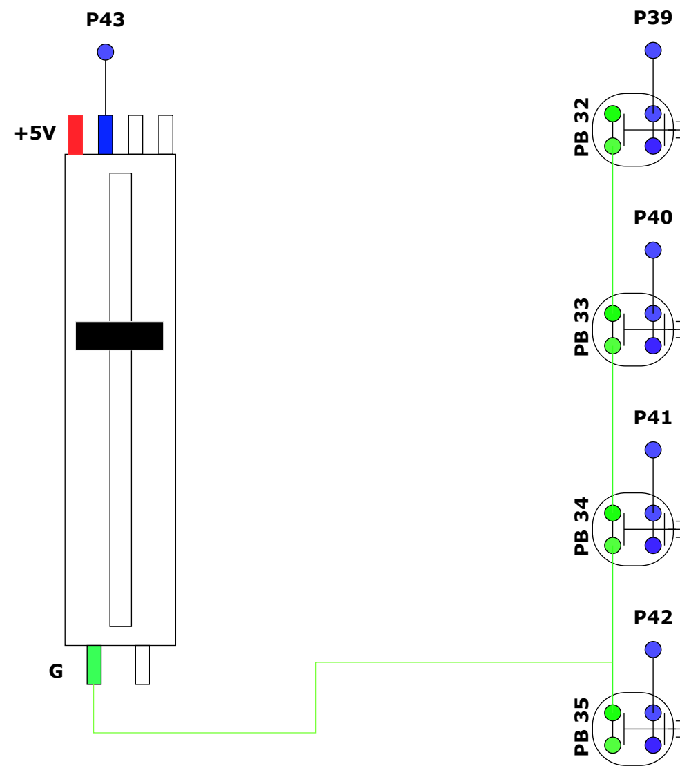
Slide Potentiometer
